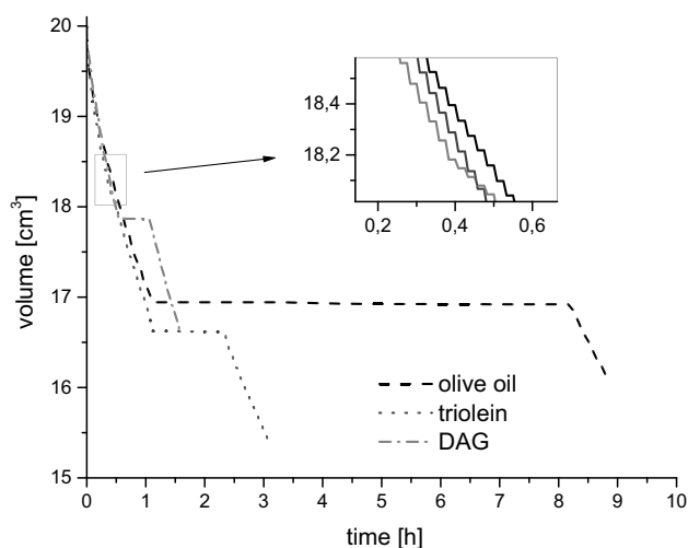
Fig. 2 Plots of the time dependences of sample volume at 20 °C
