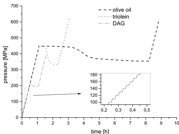
Fig. 1 Plots of the time dependences of pressure at 20 °C
